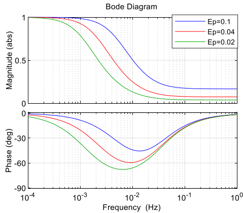
Figure 25. Varying droop with fixed parameter, same as Figure 23, scaled to have static gain = 1.
