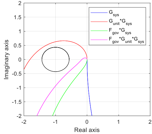
Figure 12. Nyquist diagram of the same systems as in Figure 11.
