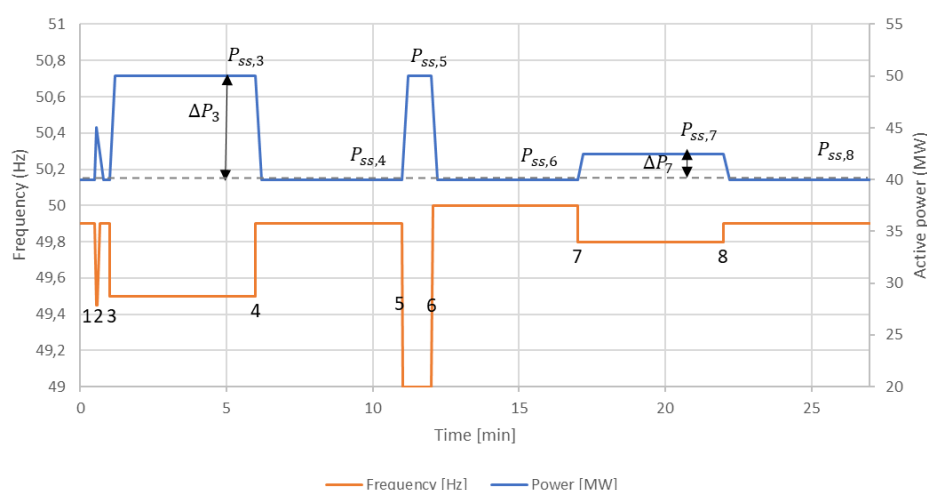
Figure 4: FCR-D upwards fast ramp test. In this illustration FCR-N is inactive and therefore P_8 = P_6 .
