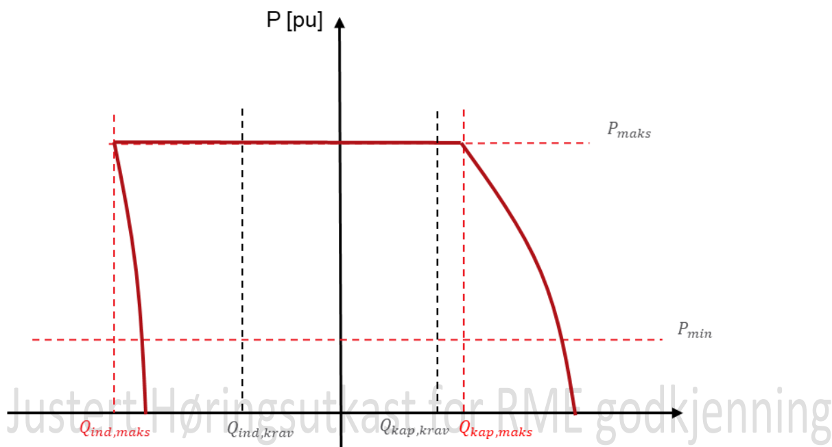
FIGUR 14-7: DRIFTSDIAGRAM FOR EN KRAFTPARK REFERERT PCC.
