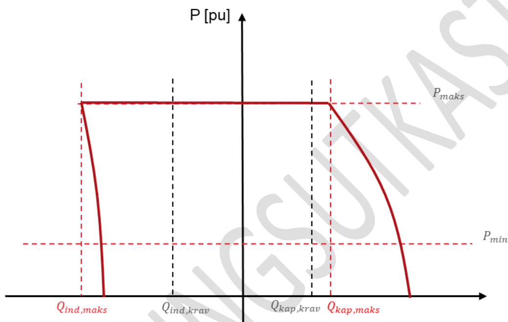
FIGUR 14-7: DRIFTSDIAGRAM FOR EN KRAFTPARK REFERERT PCC.
