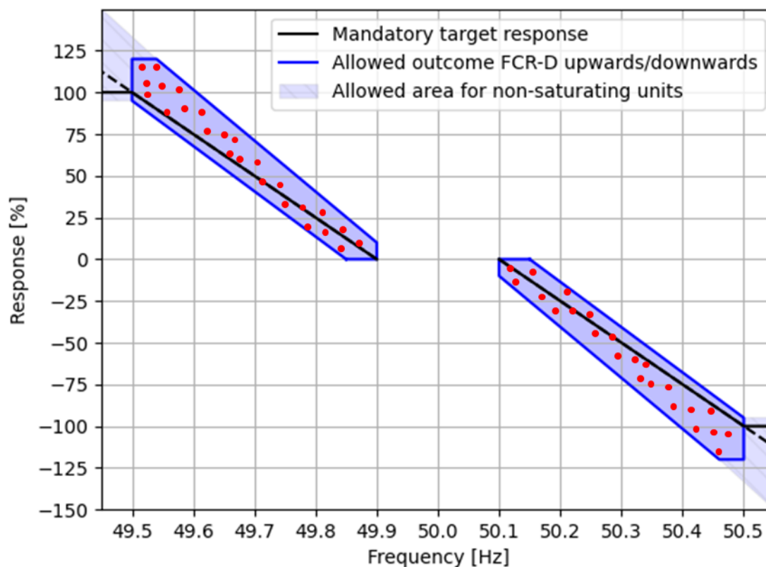
Figure 28. Example response (red dots) of stationary activation of FCR-D upwards and FCR-D downwards for an FCR providing entity, compared to requirement for linearity (blue area).
