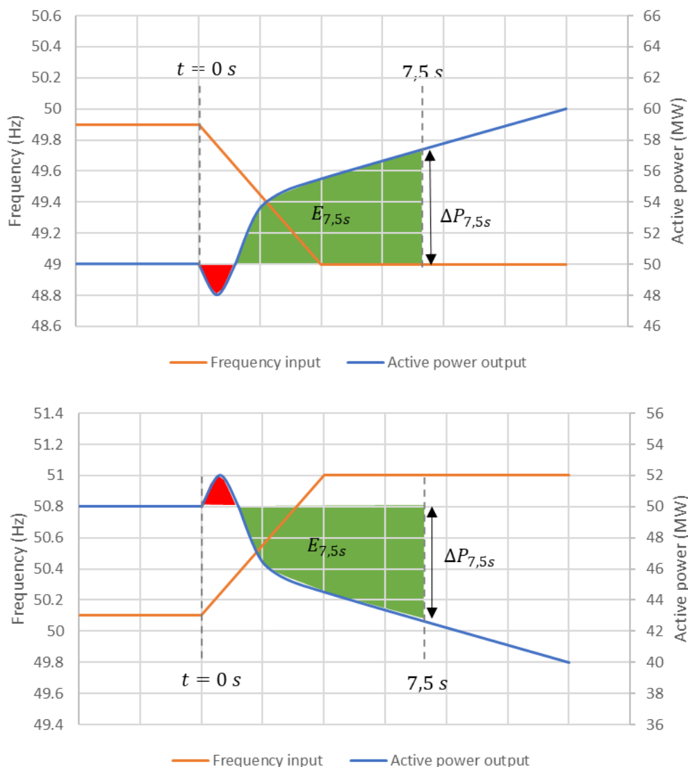
Figure 25. Calculation of FCR-D upwards capacity and FCR-D downwards capacity. The green area indicates positive energy contribution while the red area indicates negative energy contribution.
