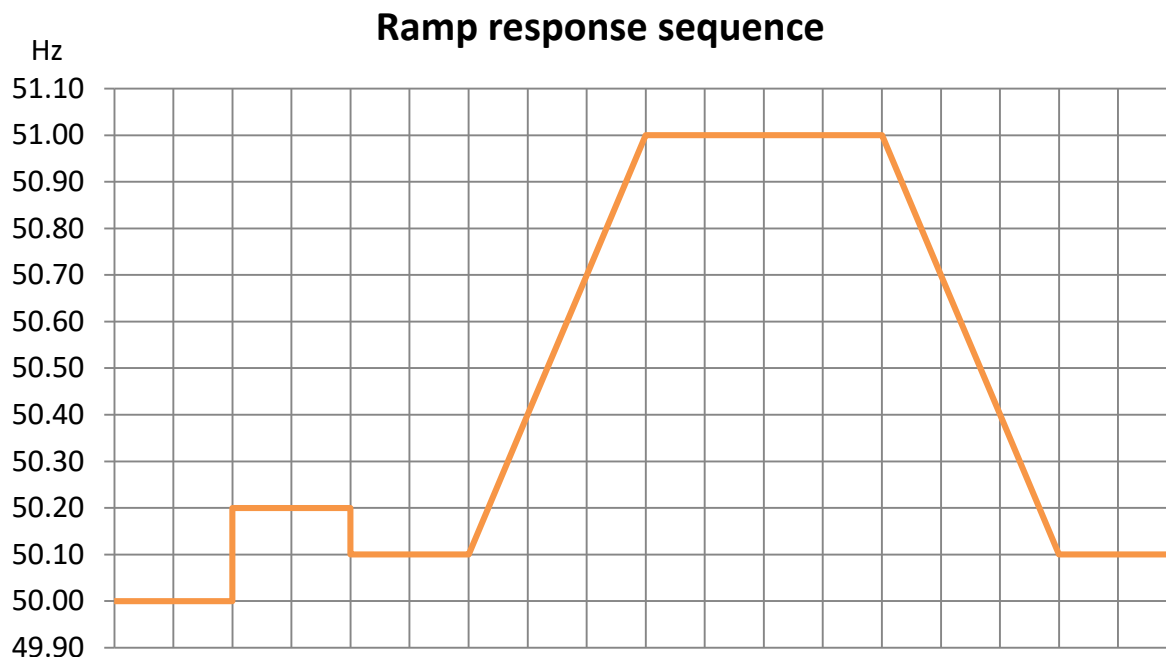
Figure 8. Input frequency signal for FCR-D downwards ramp response tests
