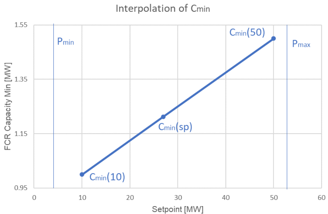
Figure 30. Second step of the linear interpolation to determine the minimal capacity for setpoints between the minimum and maximum tested setpoint.
