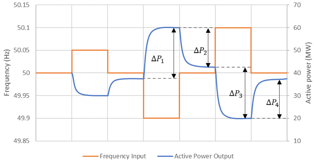
Figure 19. Example response (blue) from input frequency (orange) according to FCR-N step test
