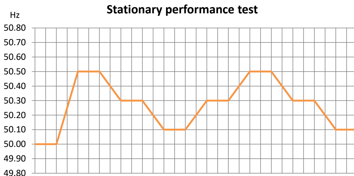
Figure 7. Input frequency signal for FCR-D downwards stationary performance response tests
