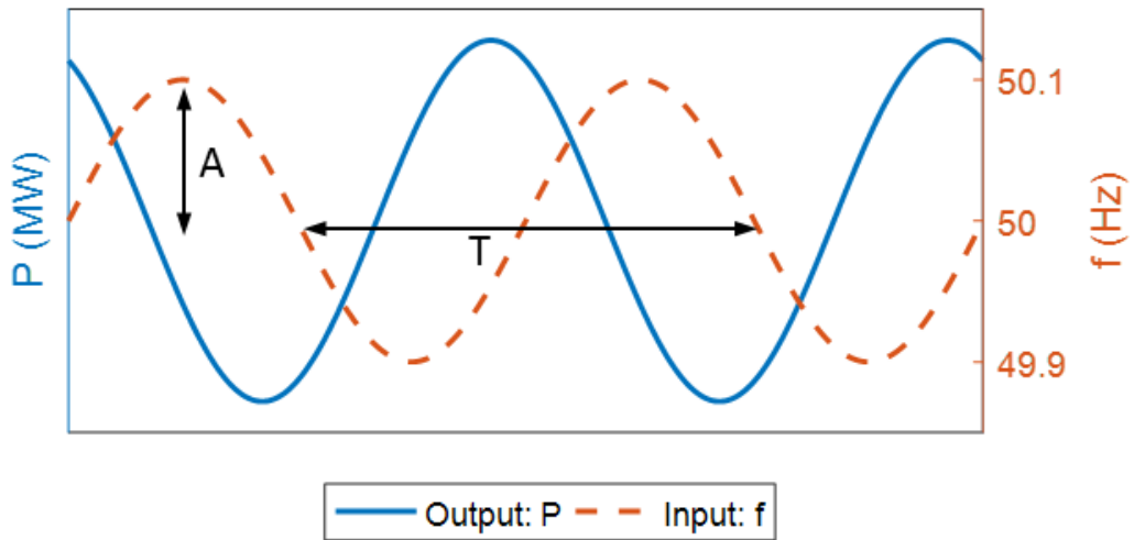
Figure 9. Input frequency signal for FCR-D sine tests
