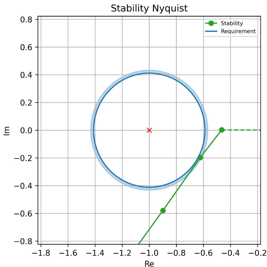
Figure 22. Nyquist diagram of the Nyquist-point (-1,0), FCR-N stability margin requirement (blue) together with an example response (green).
