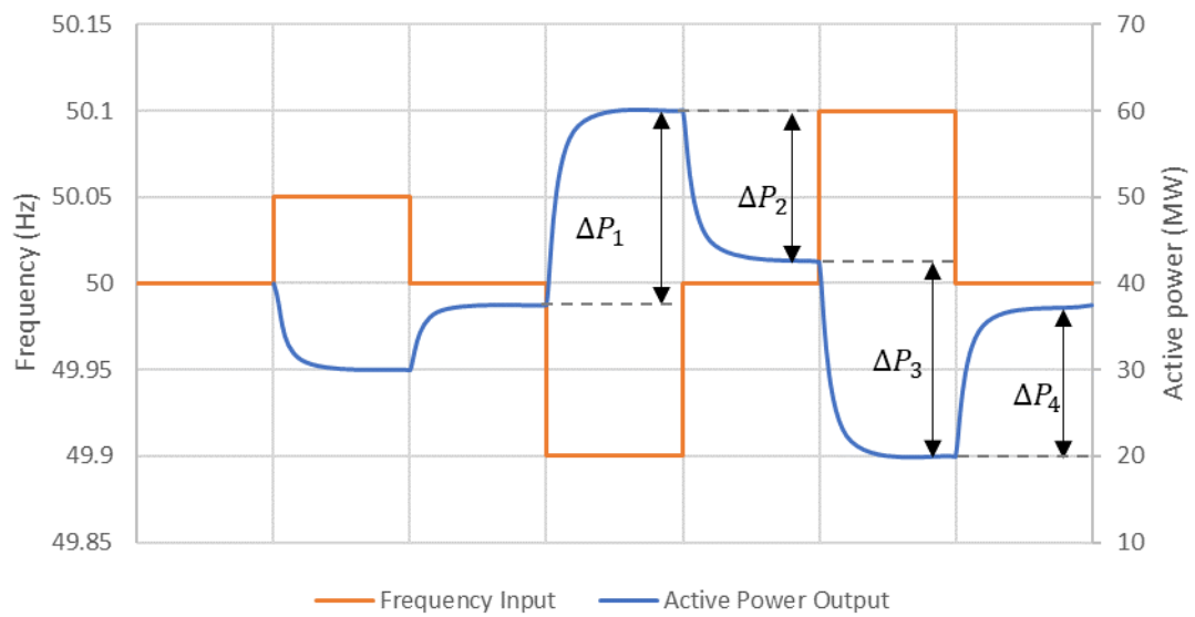
Figure 13. Example response (blue) from input frequency (orange) according to FCR-N step test.
