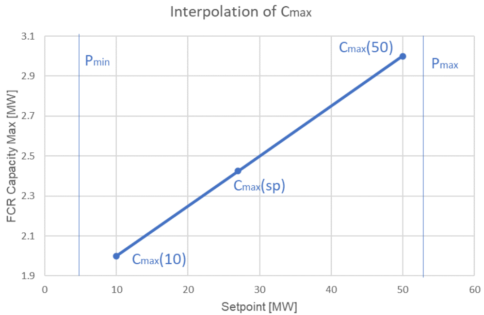
Figure 29. First step of the linear interpolation to determine the maximal capacity for setpoints between the minimum and maximum tested setpoint.
