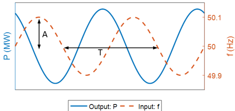
Figure 4. Input frequency signal for FCR-N sine tests
