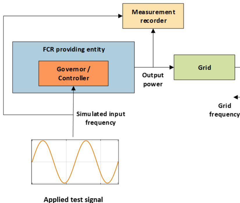
Figure 2. Principle test setup.
