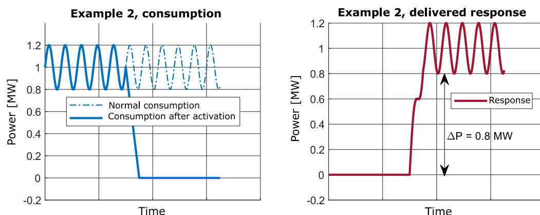
Figure 33. Example response where the variations are not independent of the delivered response.
