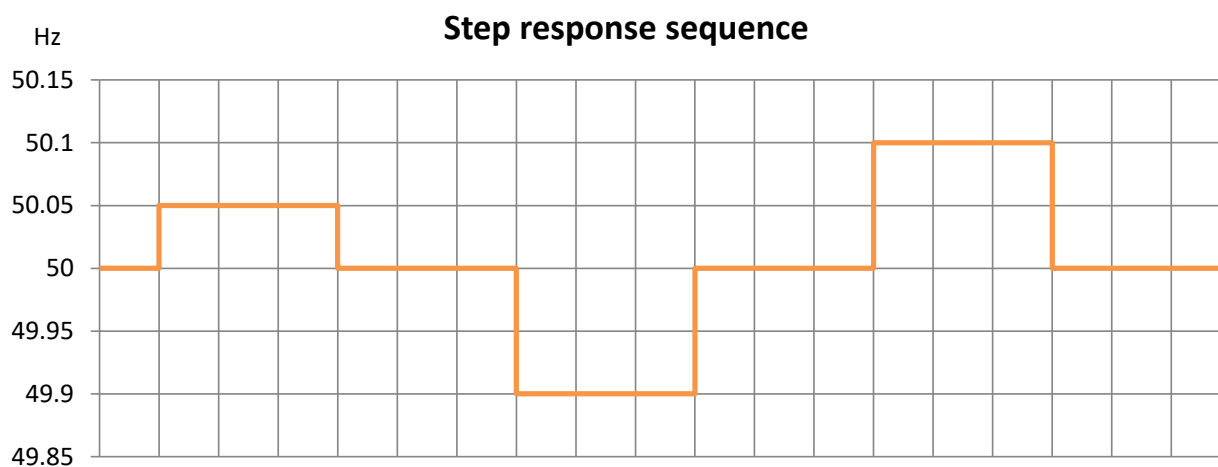
Figure 3. Input frequency signal for FCR-N step response tests
