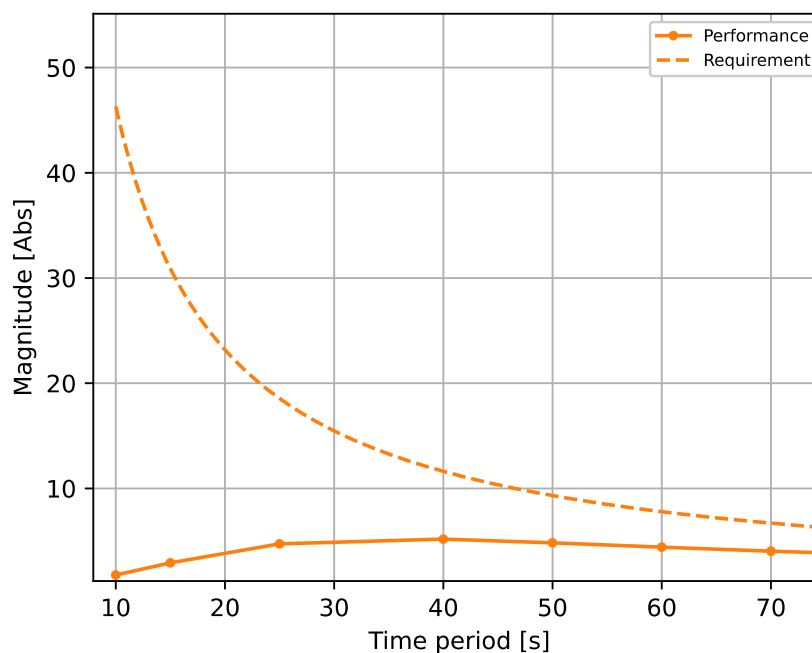
Figure 18. Example response of transfer function values (orange dots), transfer function (orange solid line) of the closed loop response, given by second column of Table 4, which qualifies for the performance requirement (orange dashed line), given by third column of Table 4.
