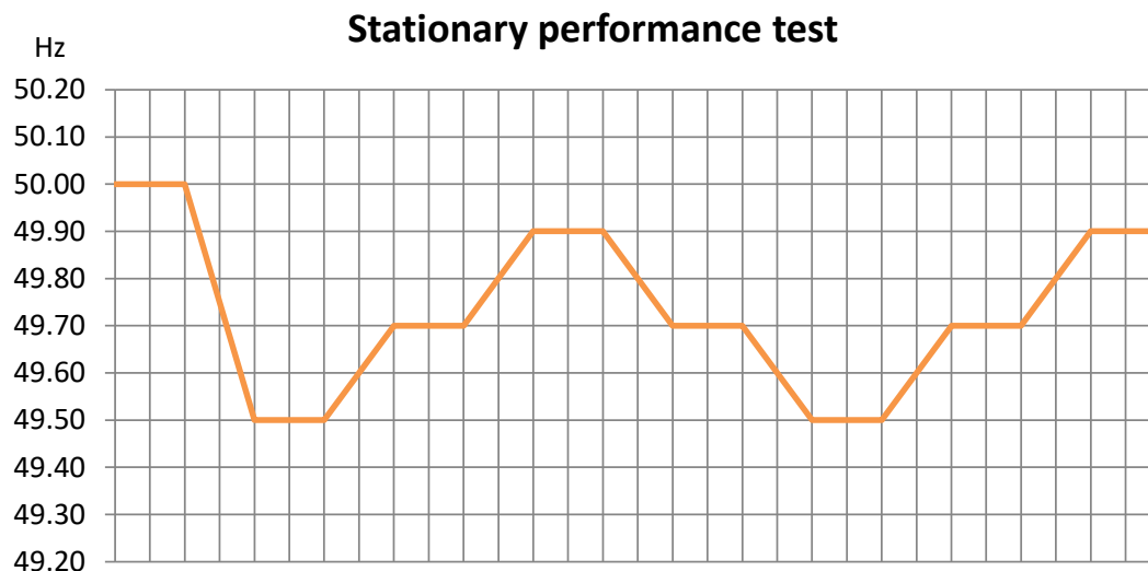
Figure 5. Input frequency signal for FCR-D upwards ramp response tests
