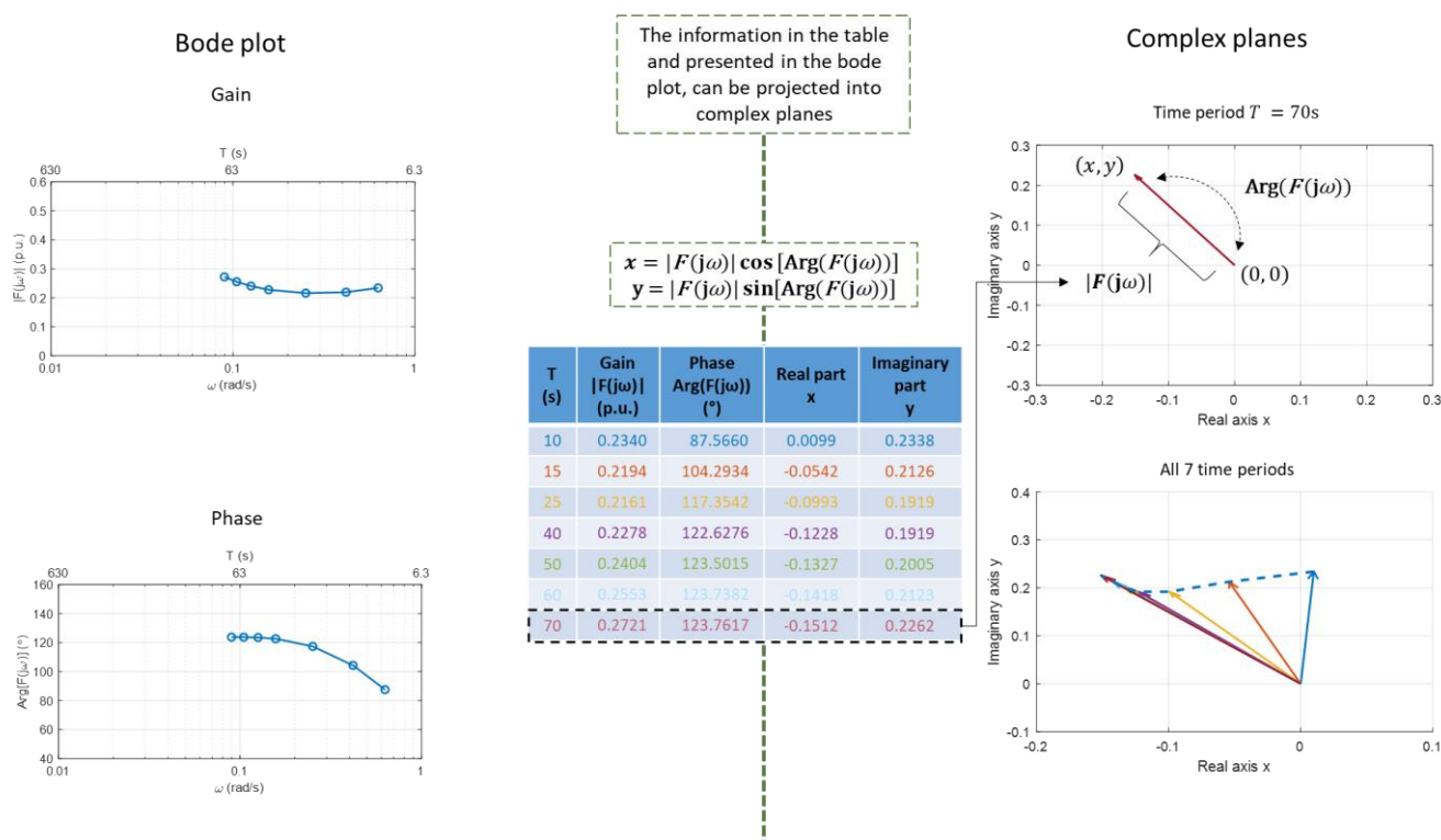
Figure 36. Bode plots, transfer function values, FCR-vectors and complex planes
