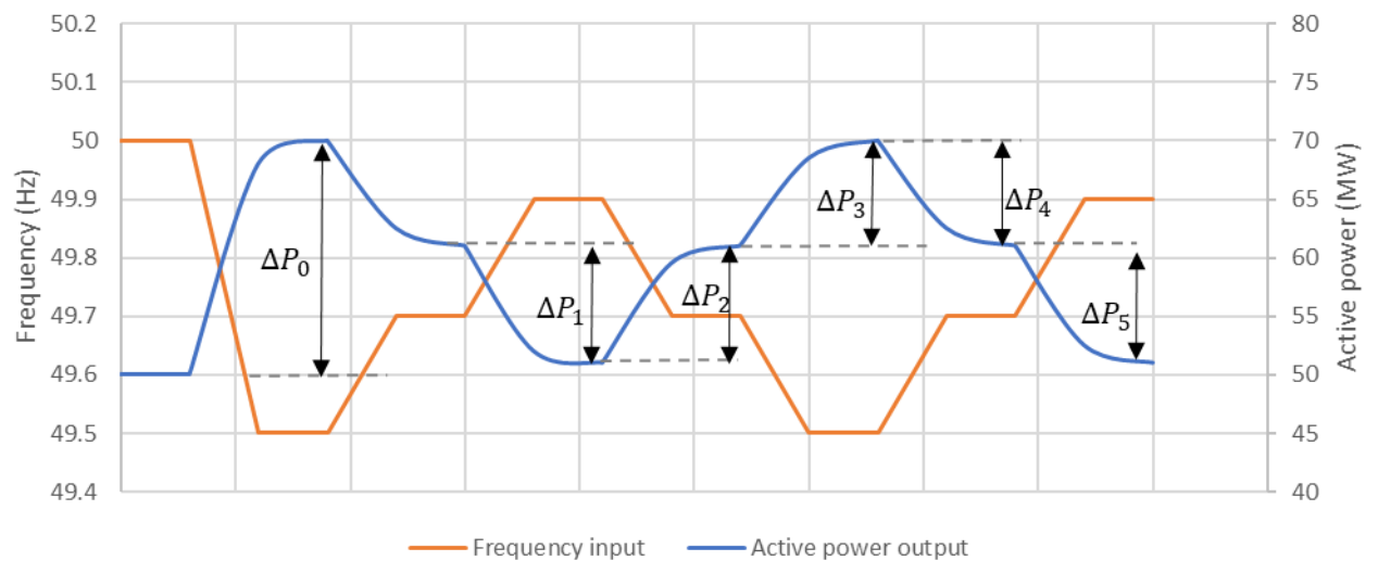
Figure 14. Example response (blue) from input frequency (orange) according to FCR-D upwards stationary performance test
