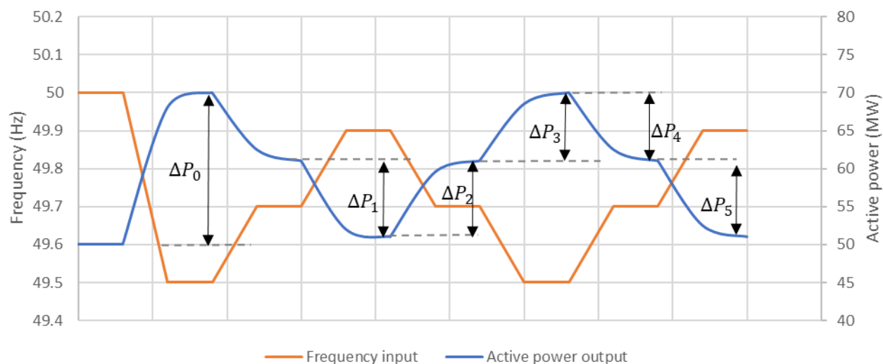
Figure 23. Example response (blue) from input frequency (orange) according to FCR-D upwards stationary performance test
