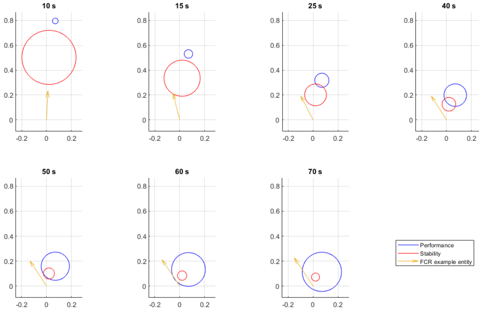
Figure 37. FCR-N dynamic performance & stability requirement circles and FCR-vectors of an example entity
