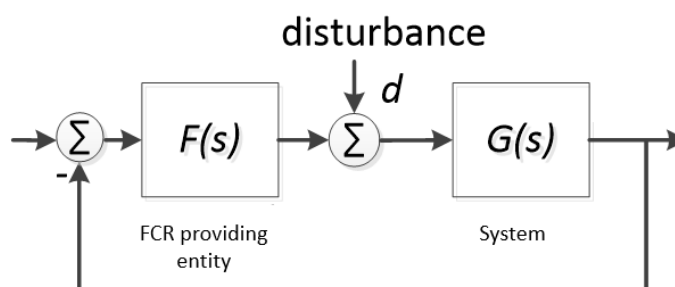
Figure 12: Illustration of the system used for evaluation of compliance with requirements in frequency domain.
