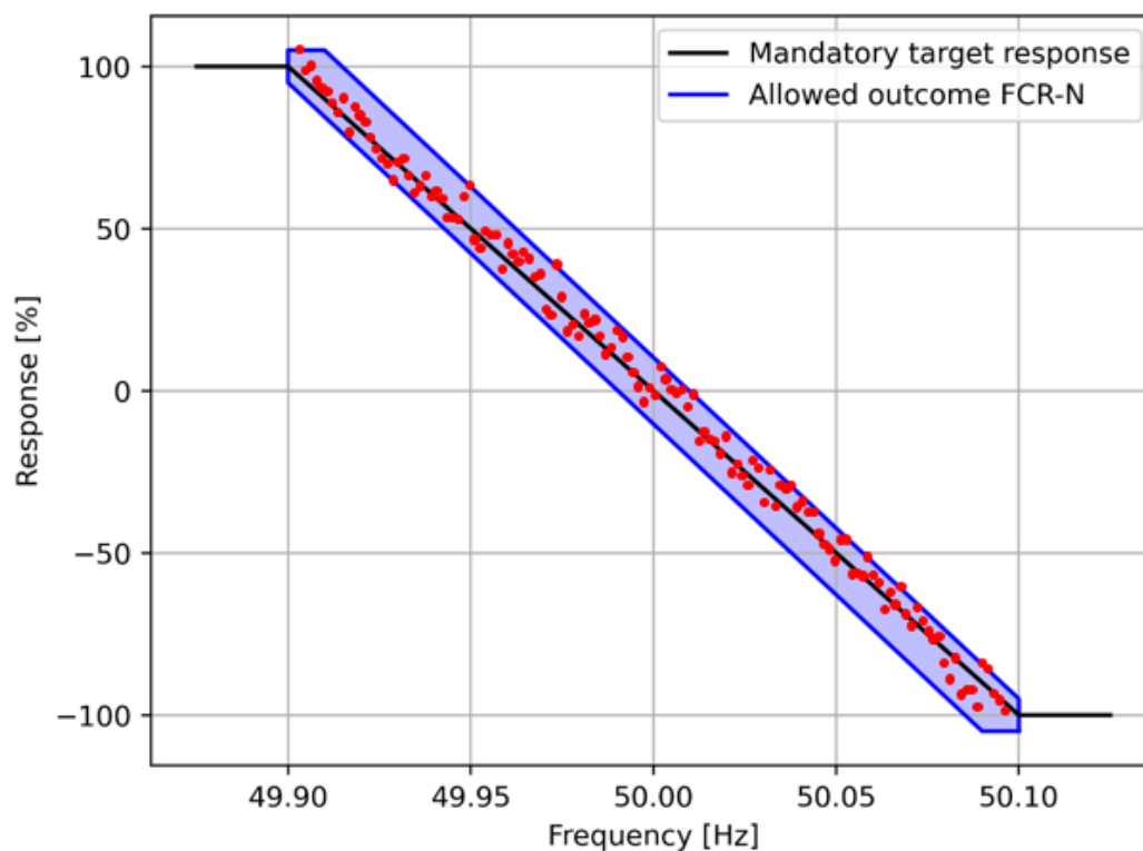
Figure 27. Example response (red dots) of stationary activation of FCR-N for an FCR providing entity, compared to requirement for linearity (blue area).
