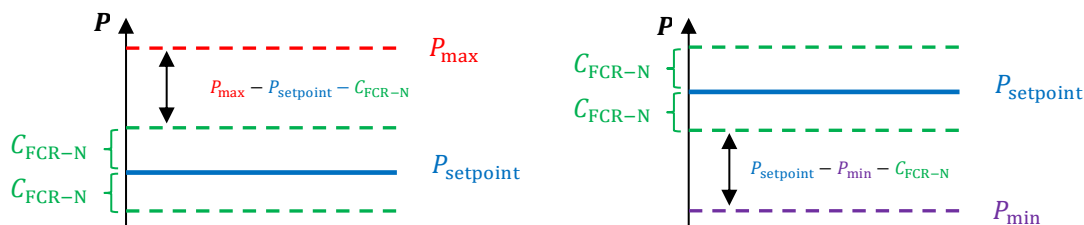
Figure 35. The limits of FCR-D capacity for a unit which is limited either by maximum active power or minimum active power while delivering FCR-N (FCR-D upwards in the left figure and FCR-D downwards in the right).
