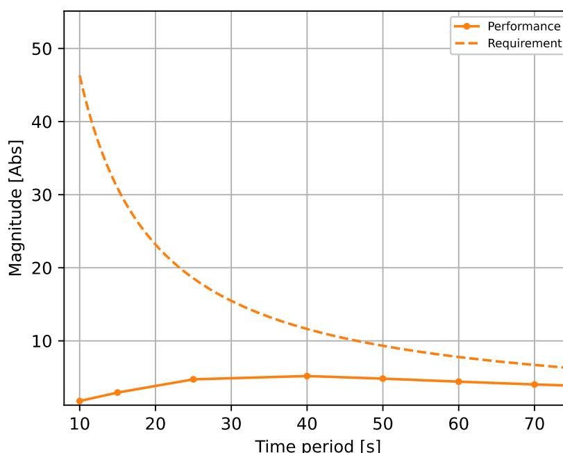
Figure 21. Example response of transfer function values (orange dots), transfer function (orange solid line) of the closed loop response which qualifies for the performance requirement (orange dashed line).
