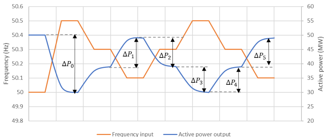
Figure 15. Example response (blue) from input frequency (orange) according to FCR-D downwards stationary performance test.
