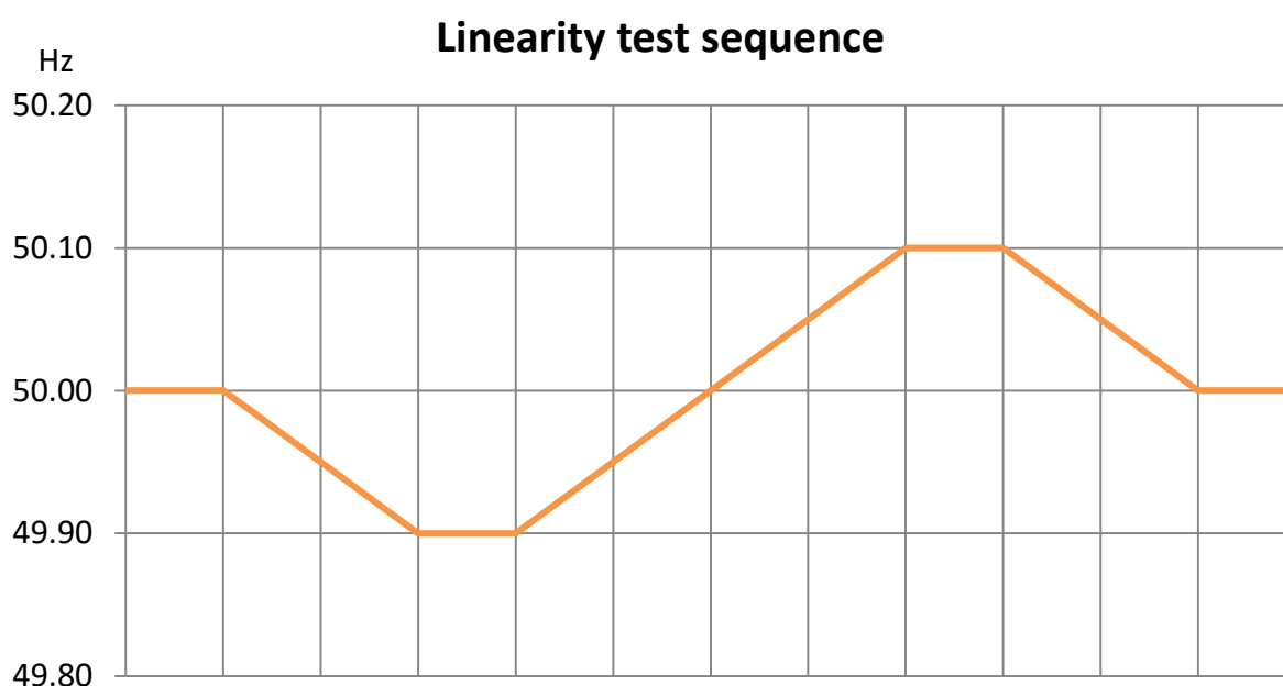
Figure 11. FCR-N linearity test sequence to be performed for minimum and maximum capacity.
