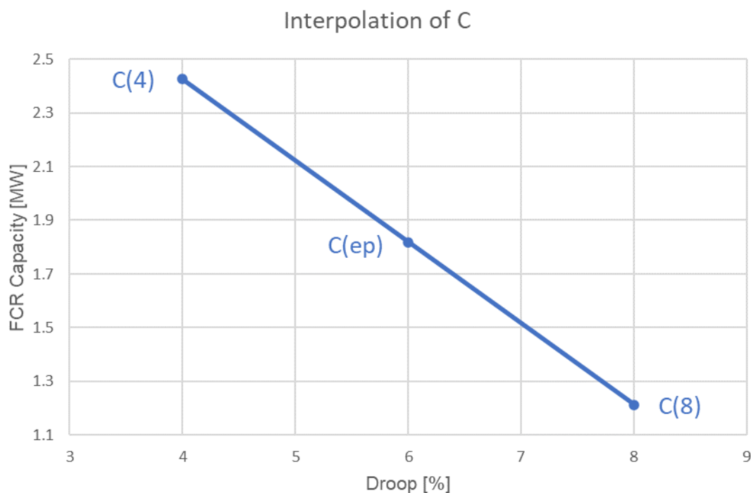
Figure 31. Third step of the linear interpolation to determine the actual capacity for droop levels between the minimum and maximum tested droop.
