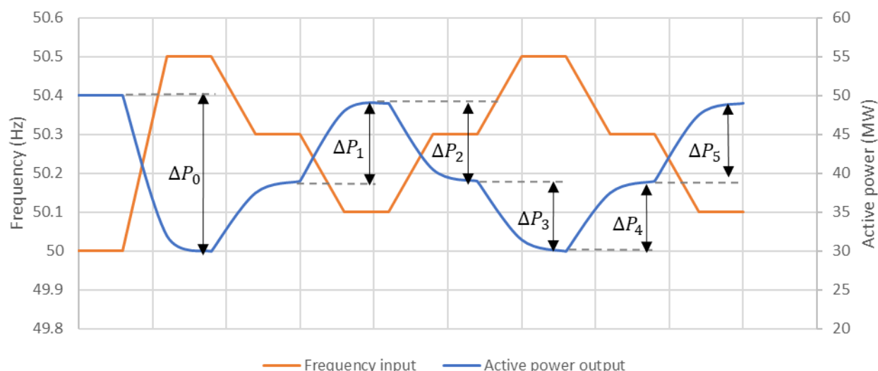
Figure 24: Example response (blue) from input frequency (orange) according to FCR-D downwards stationary performance test
