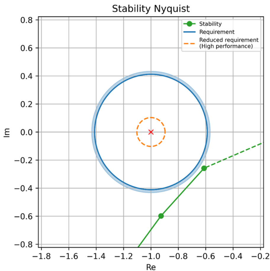
Figure 26. Illustration of FCR-D stability requirement (blue) together with an example response (green). The example response fulfils the stability requirement since it does not enter the blue circle or encircle the red cross. The orange circle indicates the reduced stability requirement for entities utilising high performance parameters in accordance with subsection 3.3.3.
