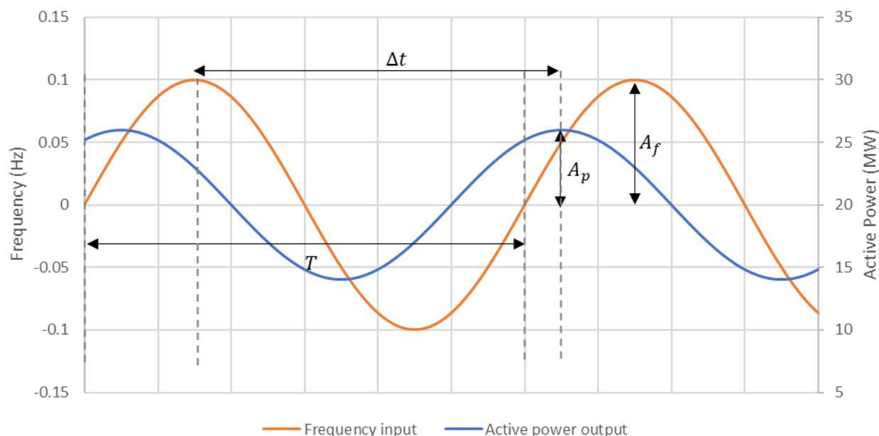
Figure 16. Example response (blue) from input frequency (orange) for FCR sine test
