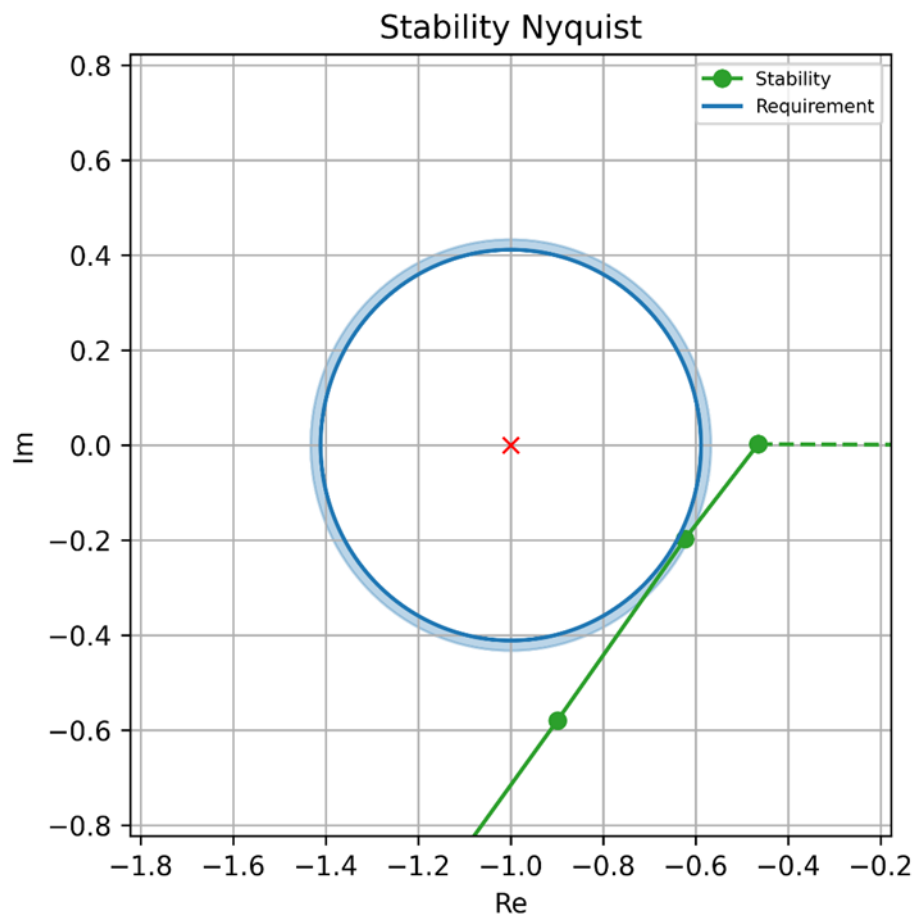
Figure 17. Example response of transfer function values (green dots) and transfer function (green line) of the open loop response, given by second and third column of Table 3, which qualifies for the stability margin requirement (blue circle of radius r = \frac{1}{M_{s,req}} = 0.43 ) and does not enclose the point (-1,0) (red cross).
