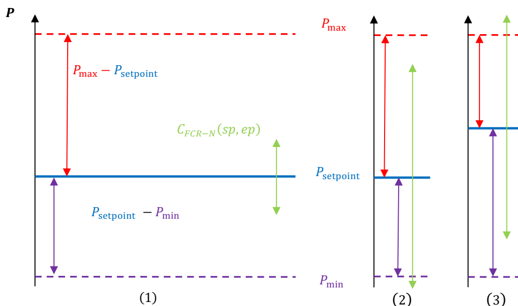
Figure 34. The three limits of FCR-N capacity for a unit which is limited either by prequalification test result (1), minimum active power (2) or maximum active power (3).
