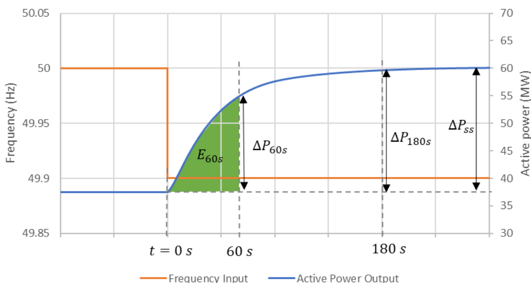
Figure 20. Example response of a single step, blue, from input frequency, orange, according to FCR-N step test from 50 to 49.9 Hz
