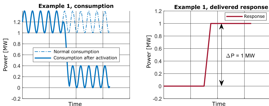
Figure 32. Example response where variations are independent of the delivered response.
